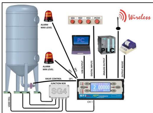
WEIGHING system of a silo.
