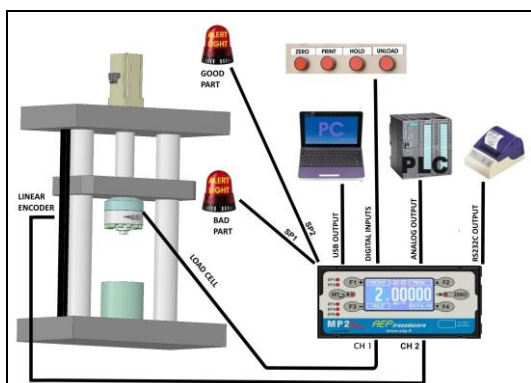
Measurement system on the press with direct control of FORCE and DISPLACEMENT (ENCODER)
