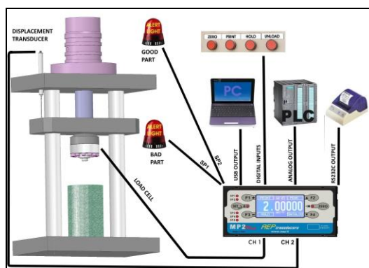
Measurement system on the press with direct control of FORCE and DISPLACEMENT
